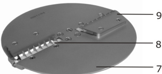
Streifenschneidscheibe 2,0x2,5 / 3,5x3,5 / 5,0x5,0 5,0x7,0 / 7,0x7,0 / 7,0x10,0
