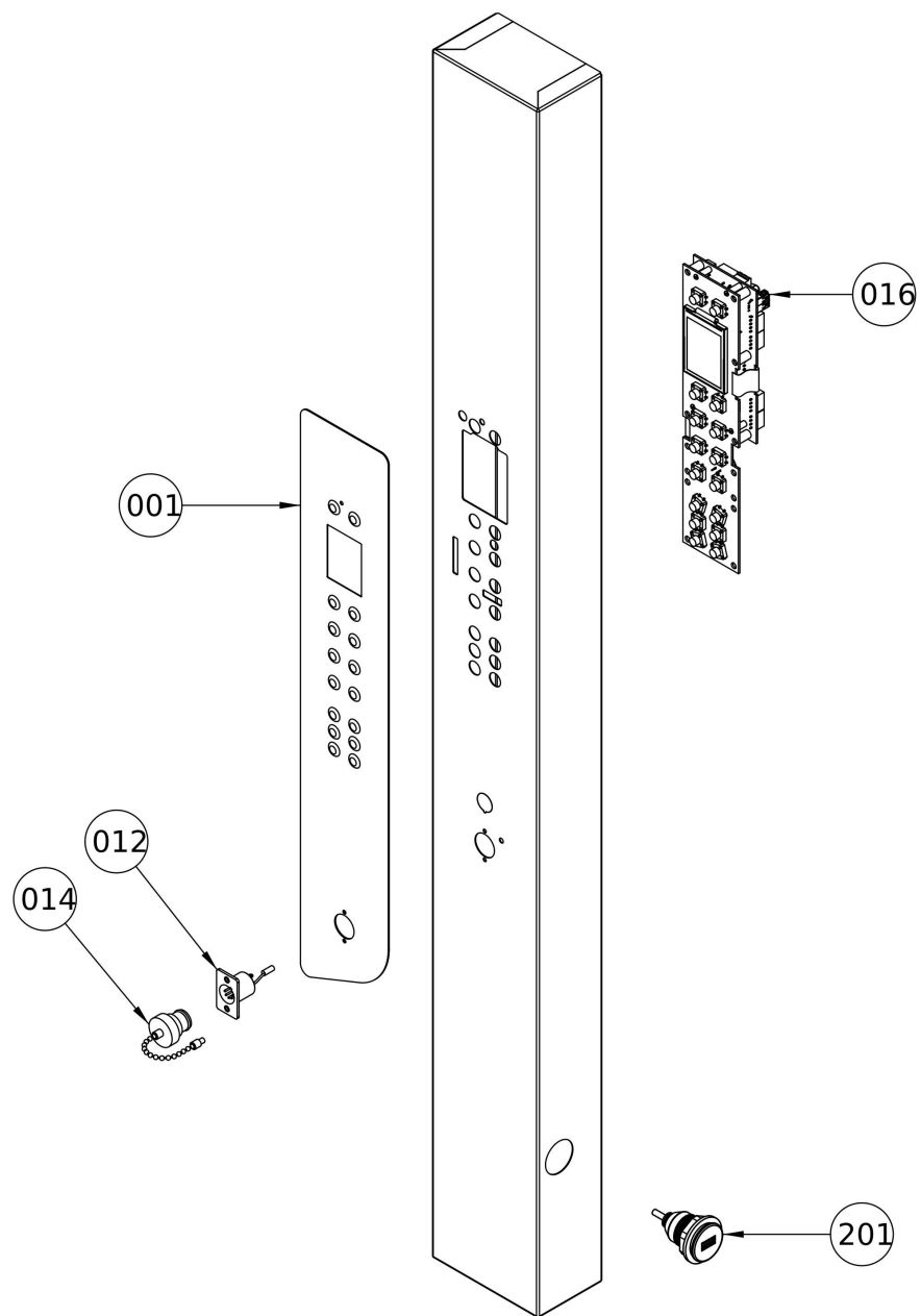
DASHBOARD PANEL
