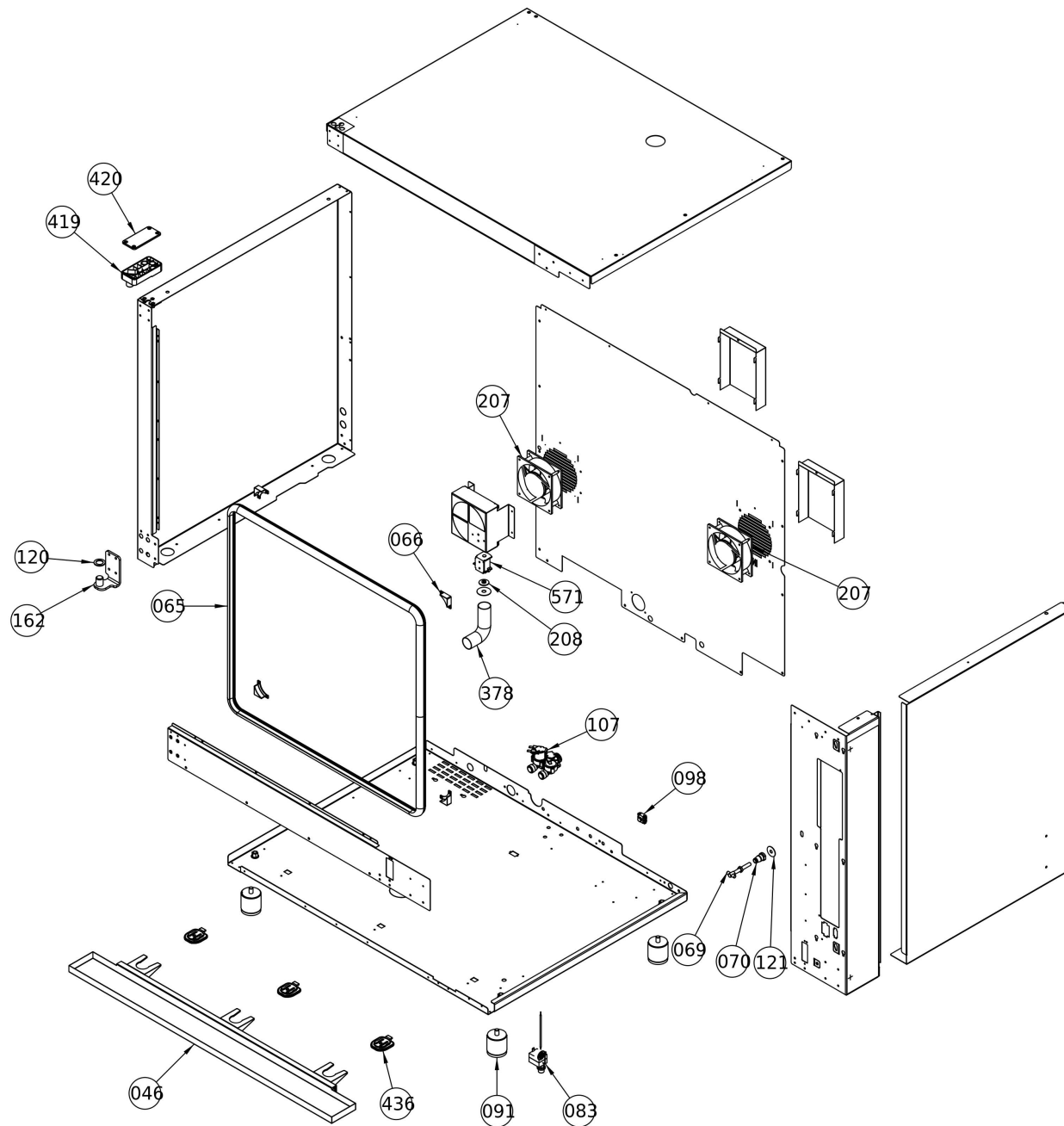
Oven body
