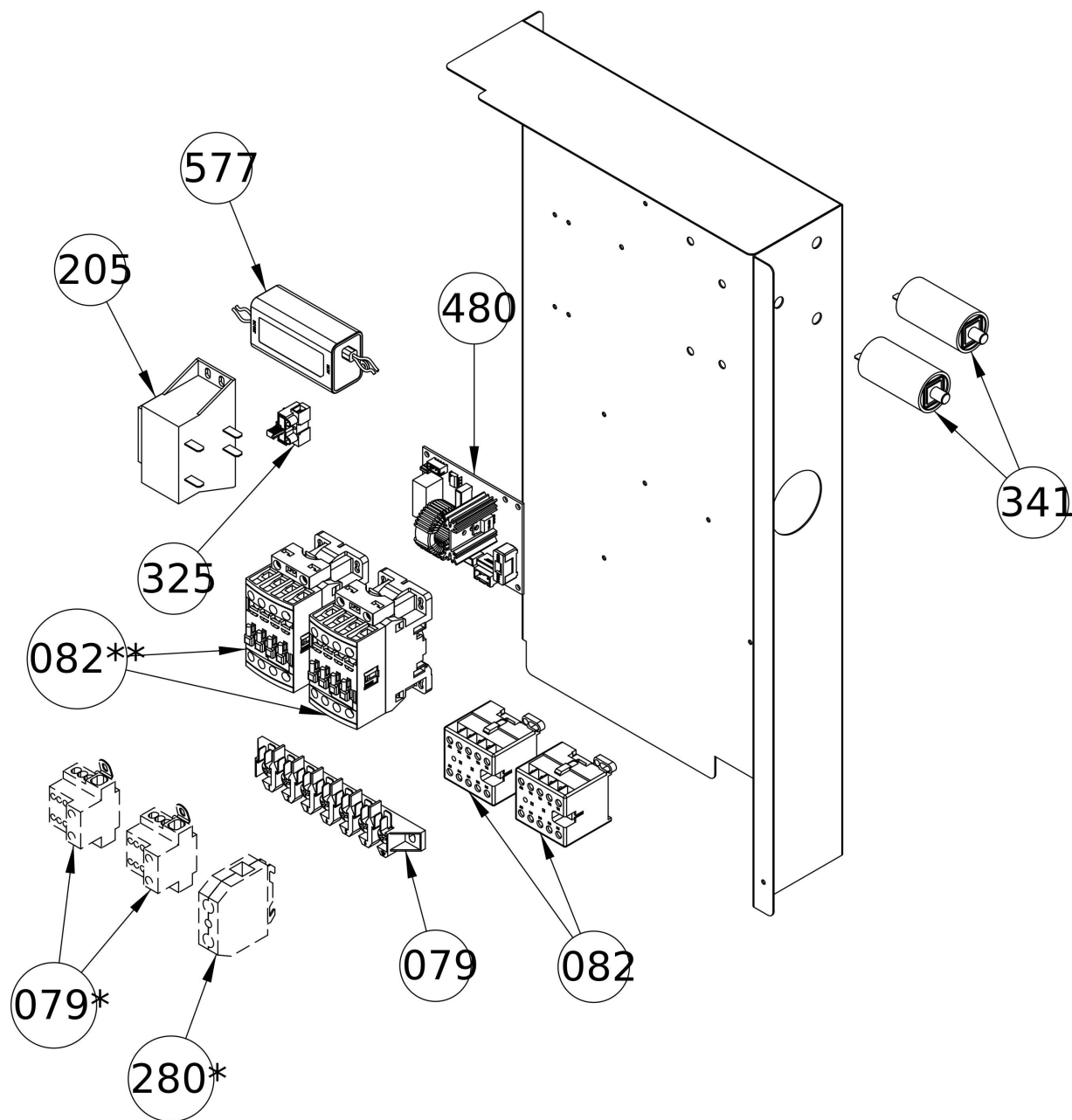
Components pannel
